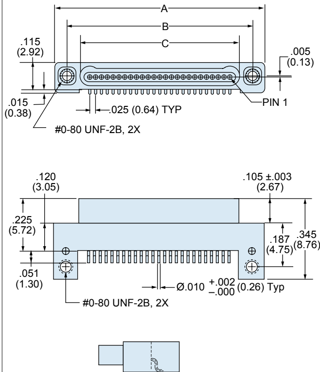
890-012 Plug (Pin) Connectors
