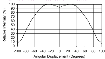
Figure 8. Representative Spatial Radiation Pattern per Luxeon emitter for Red and Amber.
