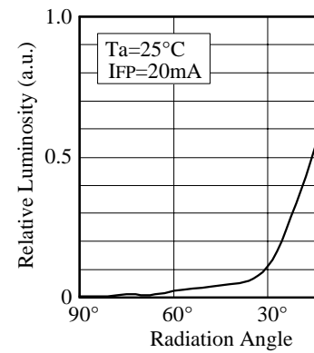
■ Directivity
