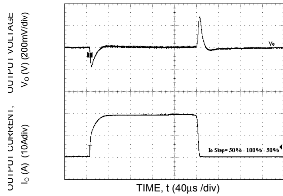
Figure 4. Transient Response to Dynamic Load Change from 0% to 50% to 100% to 50% to 0% with V_{IN}=12V .
