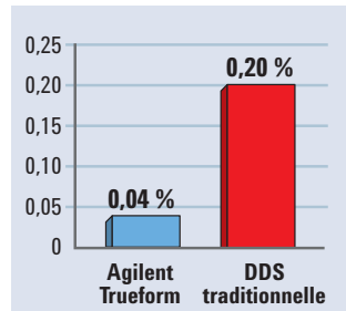
Distorsion harmonique totale
