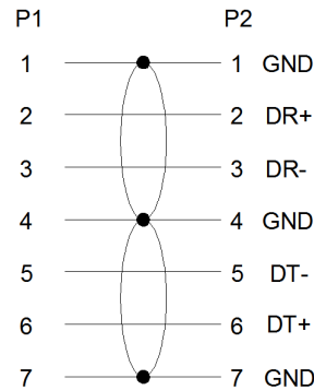
WIRING DIAGRAM
