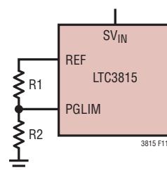
Figure 11b. PGOOD Window Set By R1/R2
