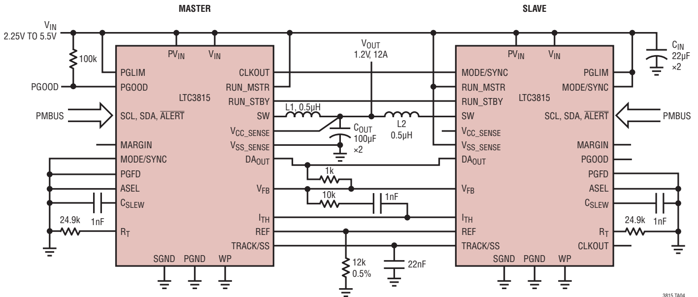
1.2V/12A 2-Phase Buck Regulator
