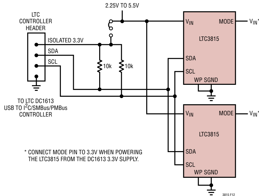
Figure 14. LTC Controller Connection
