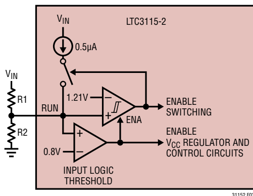
Figure 3. Accurate RUN Pin Comparator
