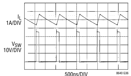
Switching Waveforms
