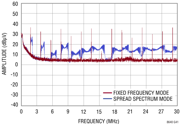
DC2202A DEMO BOARD (WITH EMI FILTER INSTALLED) 14V INPUT TO 5V OUTPUT AT 4A, f SW = 2MHz
