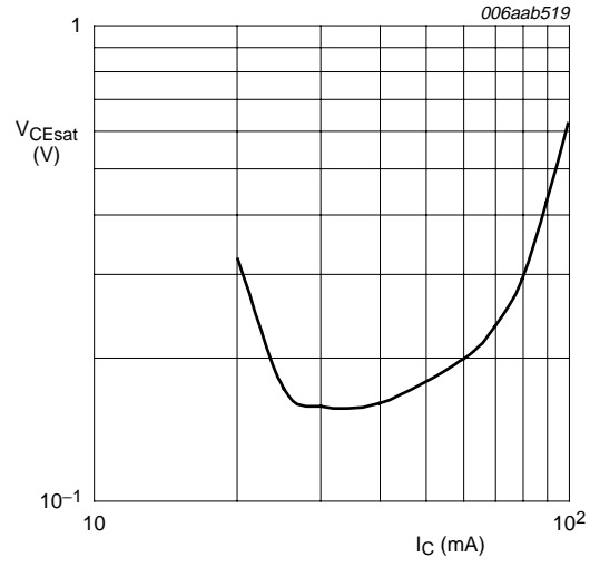
I_C/I_B = 50; T_{amb} = 25\text{ }^\circ\text{C}
