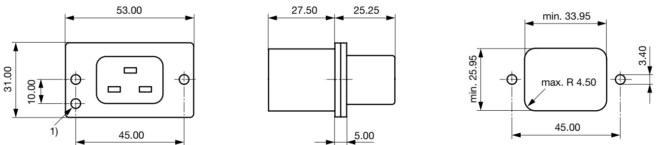
1) Orientation hole
