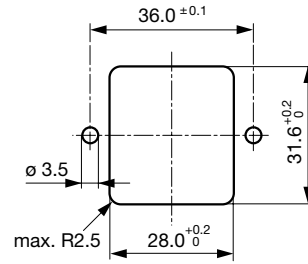
Panel cut-out for rear mounting
