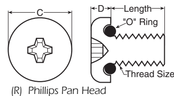
(R) Phillips Pan Head
