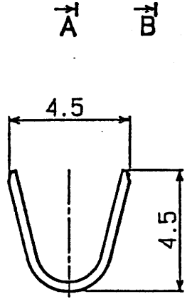
B-B SEC.
