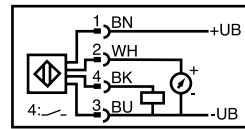
0-10v Connection
