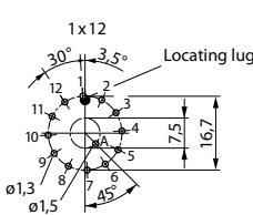
Drilling diagram for 30° indexing angle
