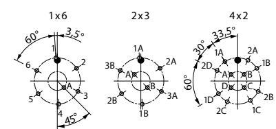
Drilling diagram for 60° indexing angle
