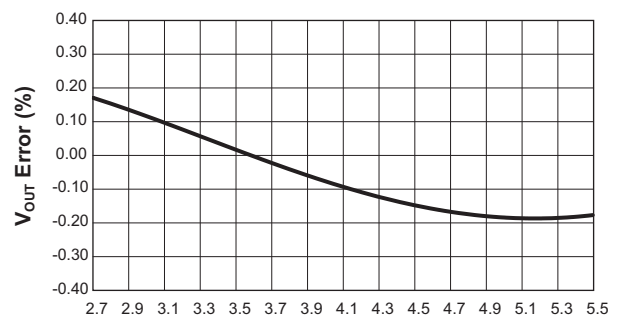
Line Regulation
