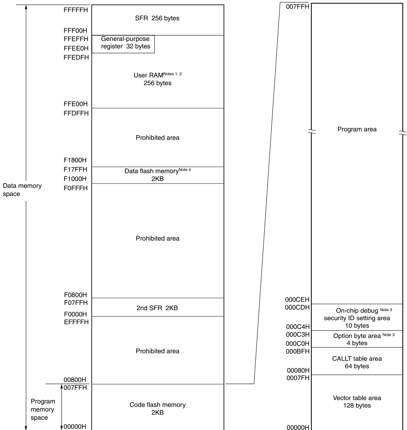
Figure 3-1. Memory Map for the R5F10266 and R5F10366
