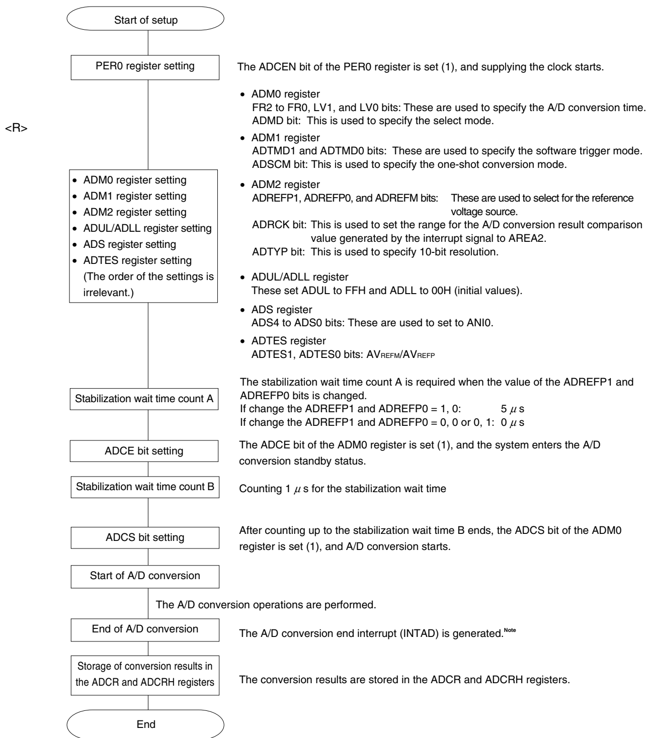
Figure 10-36. Setting up Test Trigger Mode
