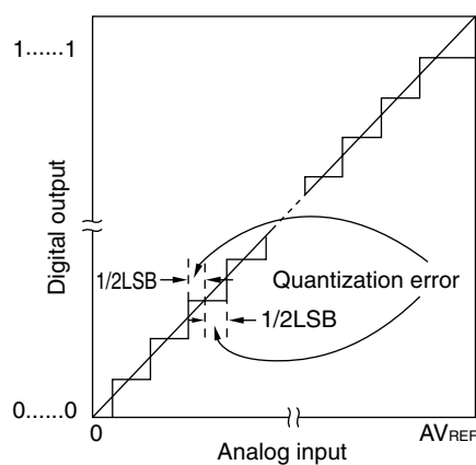
Figure 10-41. Quantization Error
