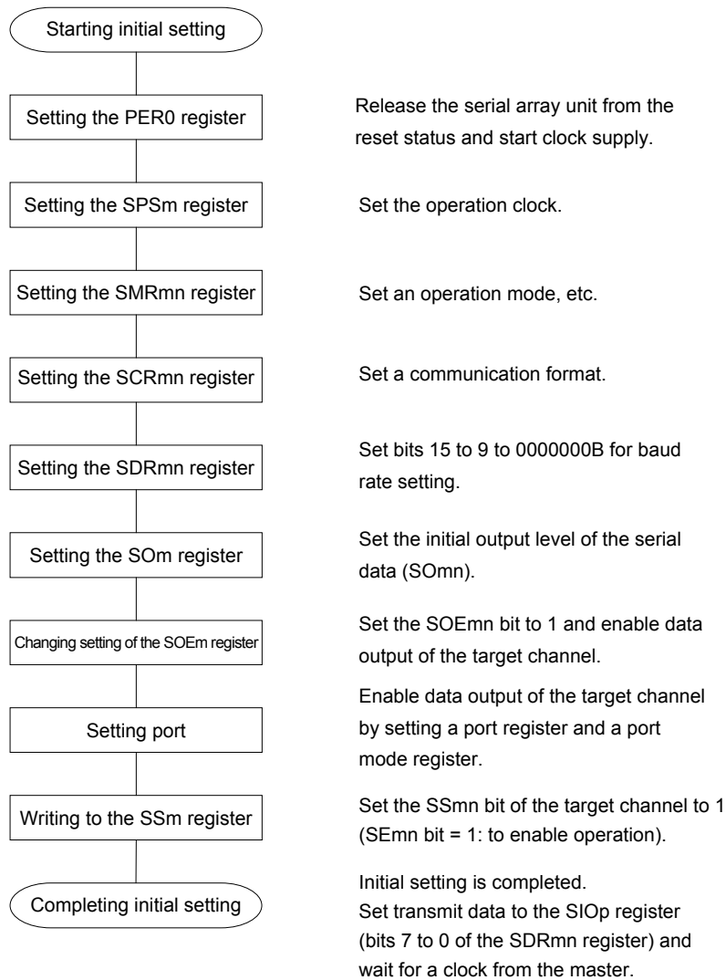
Figure 11-65. Initial Setting Procedure for Slave Transmission/Reception
