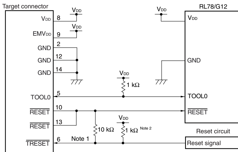
<R> Figure 25-3. Connection Example of E1 On-chip Debugging Emulator and RL78/G12 (30-pin products)
