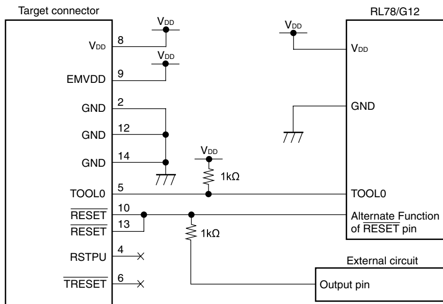
<R> Figure 25-3. Connection Example of E1 On-chip Debugging Emulator and RL78/G12 (30-pin products)
