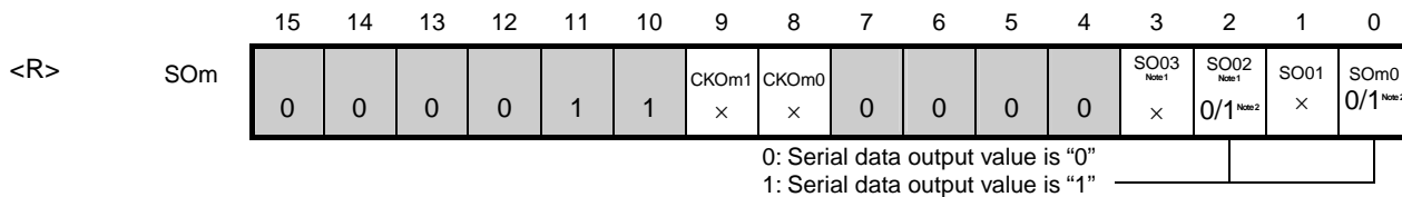
Figure 11-77. Example of Contents of Registers for UART Transmission (UART0 to UART2) (2/2)
