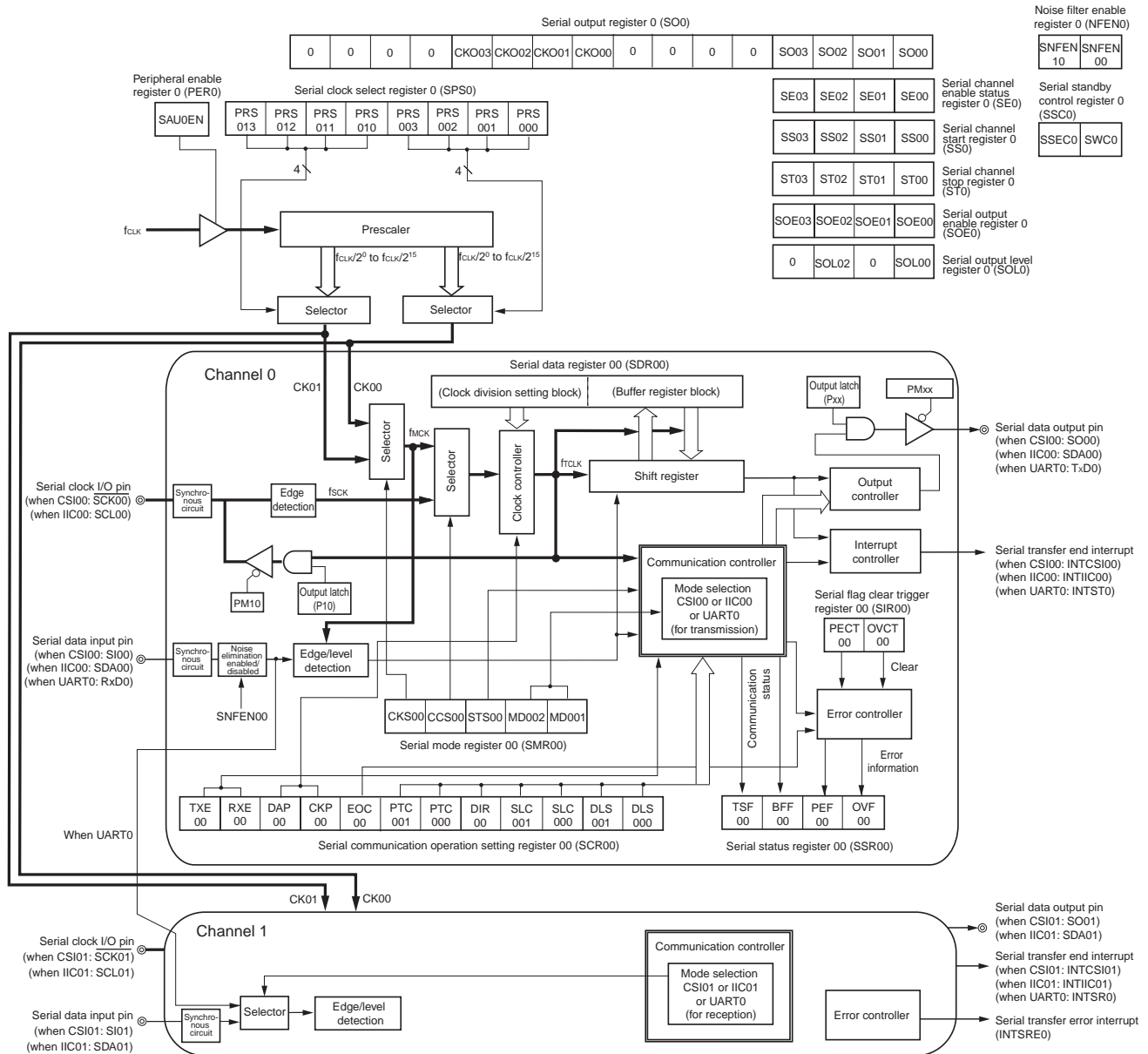
Figure 11-1. Block Diagram of Serial Array Unit 0 (20- or 24-pin products)
