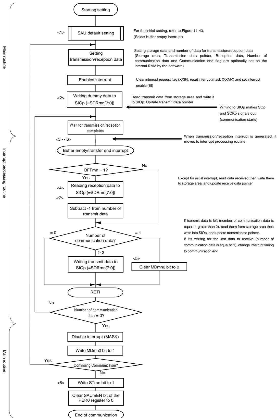
<R> Figure 11-49. Flowchart of Master Transmission/Reception (in Continuous Transmission/Reception Mode)
