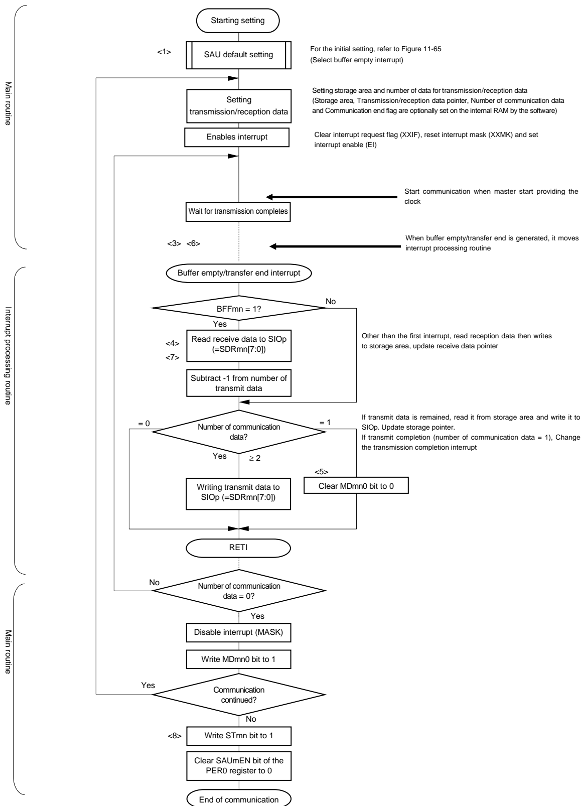
<R> Figure 11-71. Flowchart of Slave Transmission/Reception (in Continuous Transmission/Reception Mode)
