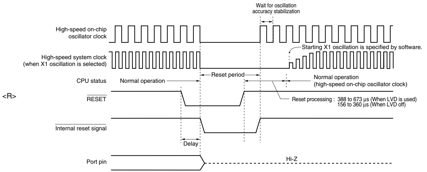
Figure 18-2. Timing of Reset by RESET Input
