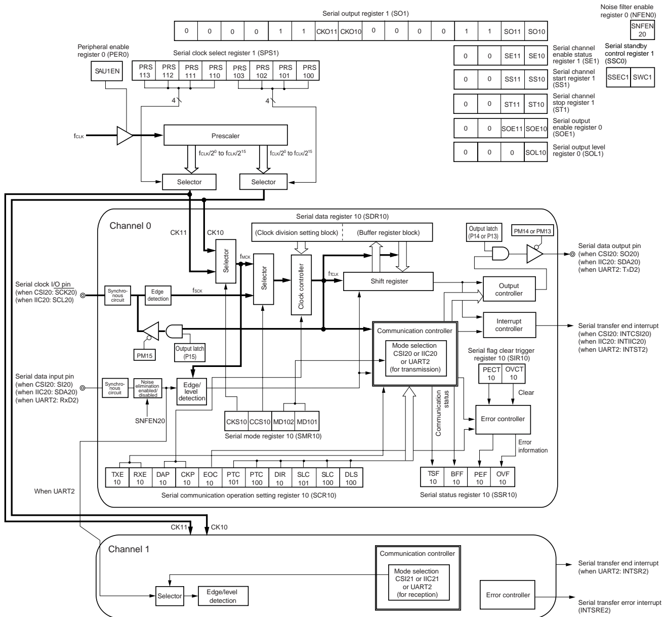
Figure 11-3. Block Diagram of Serial Array Unit 1 (30-pin products)
