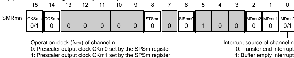
Figure 11-34. Example of Contents of Registers for Master Reception of 3-Wire Serial I/O (CSI00, CSI01, CSI11, CSI20)
