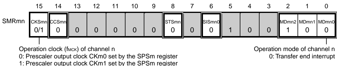
<R> Figure 11-99. Example of Contents of Registers for Address Field Transmission of Simplified I 2 C (IIC00, IIC01, IIC11, IIC20)
