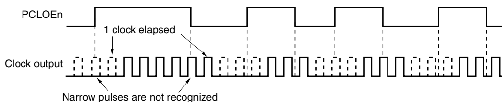
Figure 8-5. Remote Control Output Application Example
