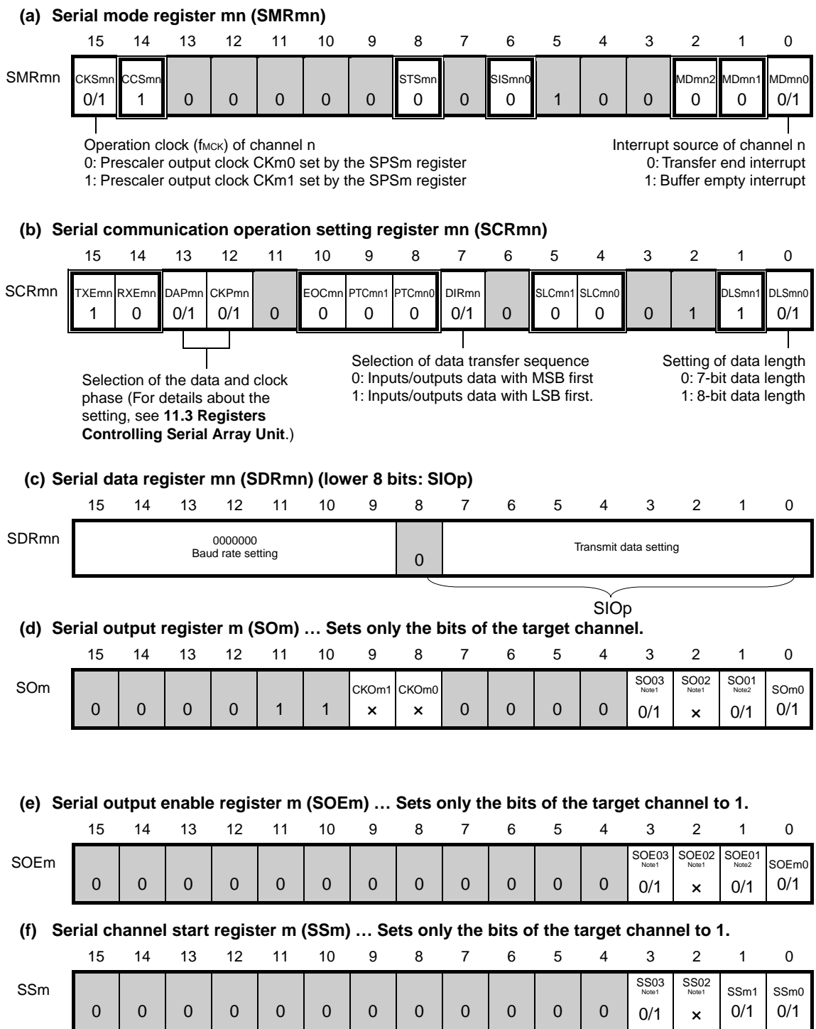
<R> Figure 11-50. Example of Contents of Registers for Slave Transmission of 3-Wire Serial I/O (CSI00, CSI01, CSI11, CSI20)
