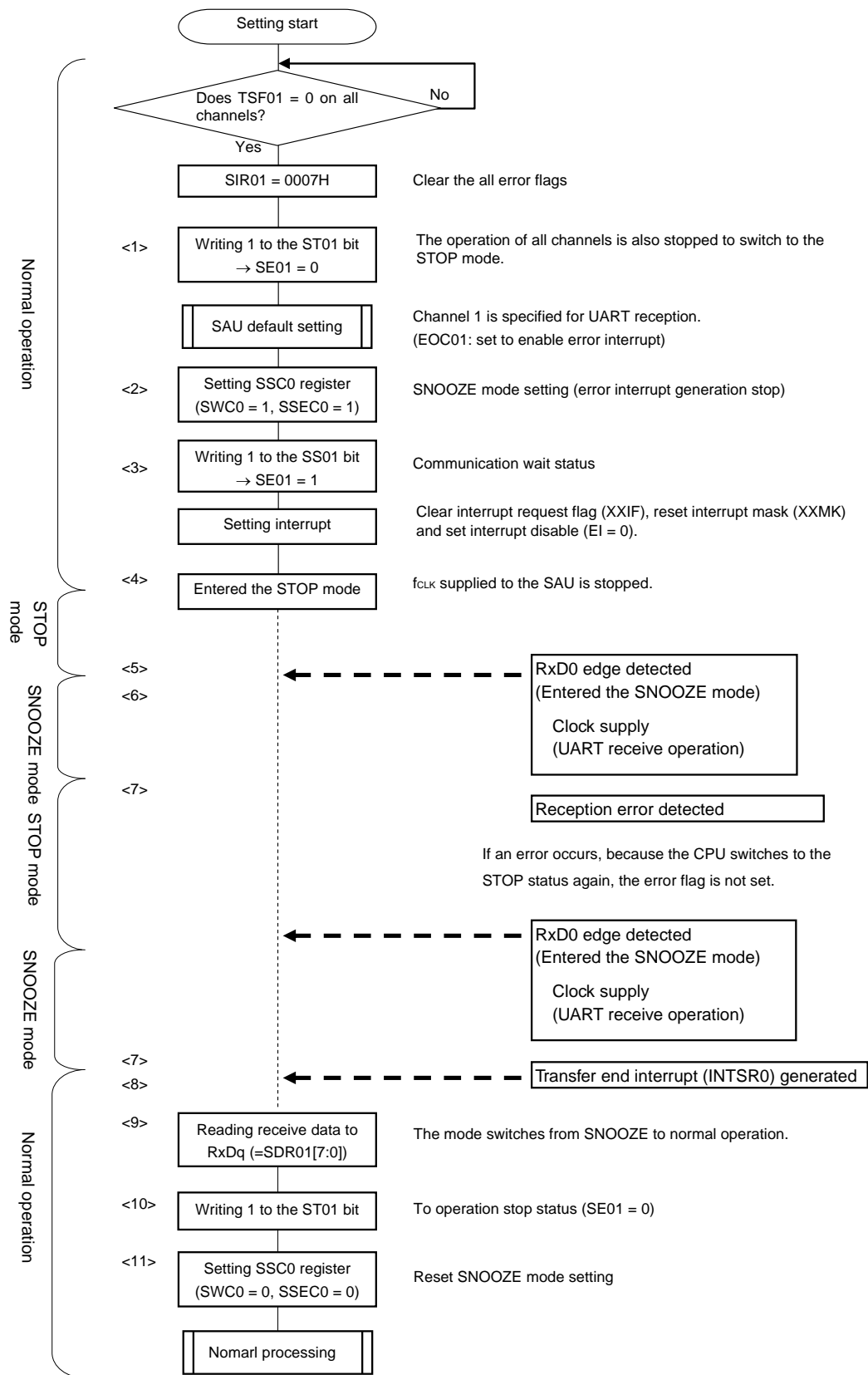
Figure 11-95. Flowchart of SNOOZE Mode Operation (Abnormal Operation <2>)
