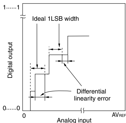
Figure 10-45. Differential Linearity Error
