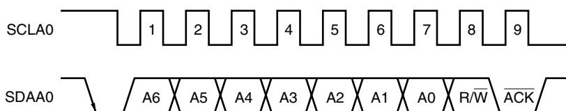
Figure 12-18. \overline{\text{ACK}}
