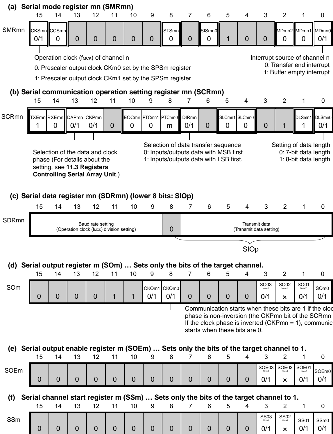
<R> Figure 11-26. Example of Contents of Registers for Master Transmission of 3-Wire Serial I/O (CSI00, CSI01, CSI11, CSI20)
