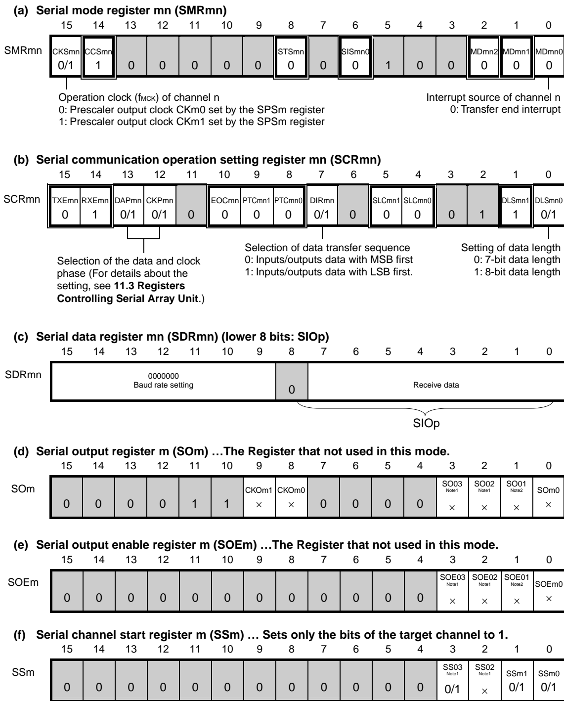
<R> Figure 11-58. Example of Contents of Registers for Slave Reception of 3-Wire Serial I/O (CSI00, CSI01, CSI11, CSI20)
