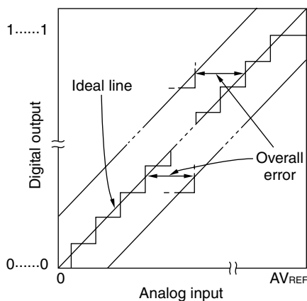
Figure 10-40. Overall Error
