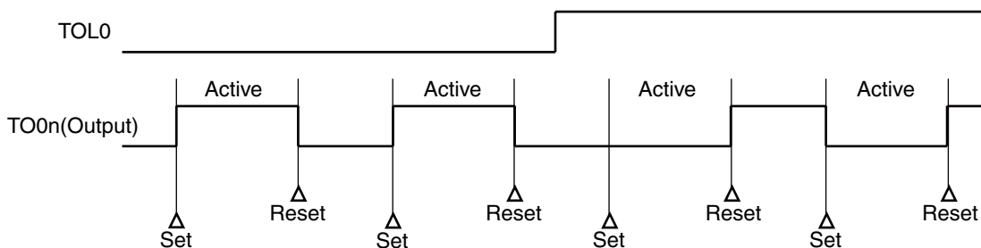
<R> Figure 6-32. Operation when TOL0 Register Has Been Changed during Timer Operation
