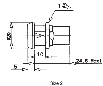
HM : Sealed Rear Mount Receptacle
