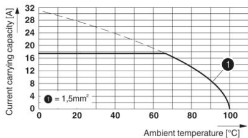
Derating diagram for 5 pins;reduction factor=1
