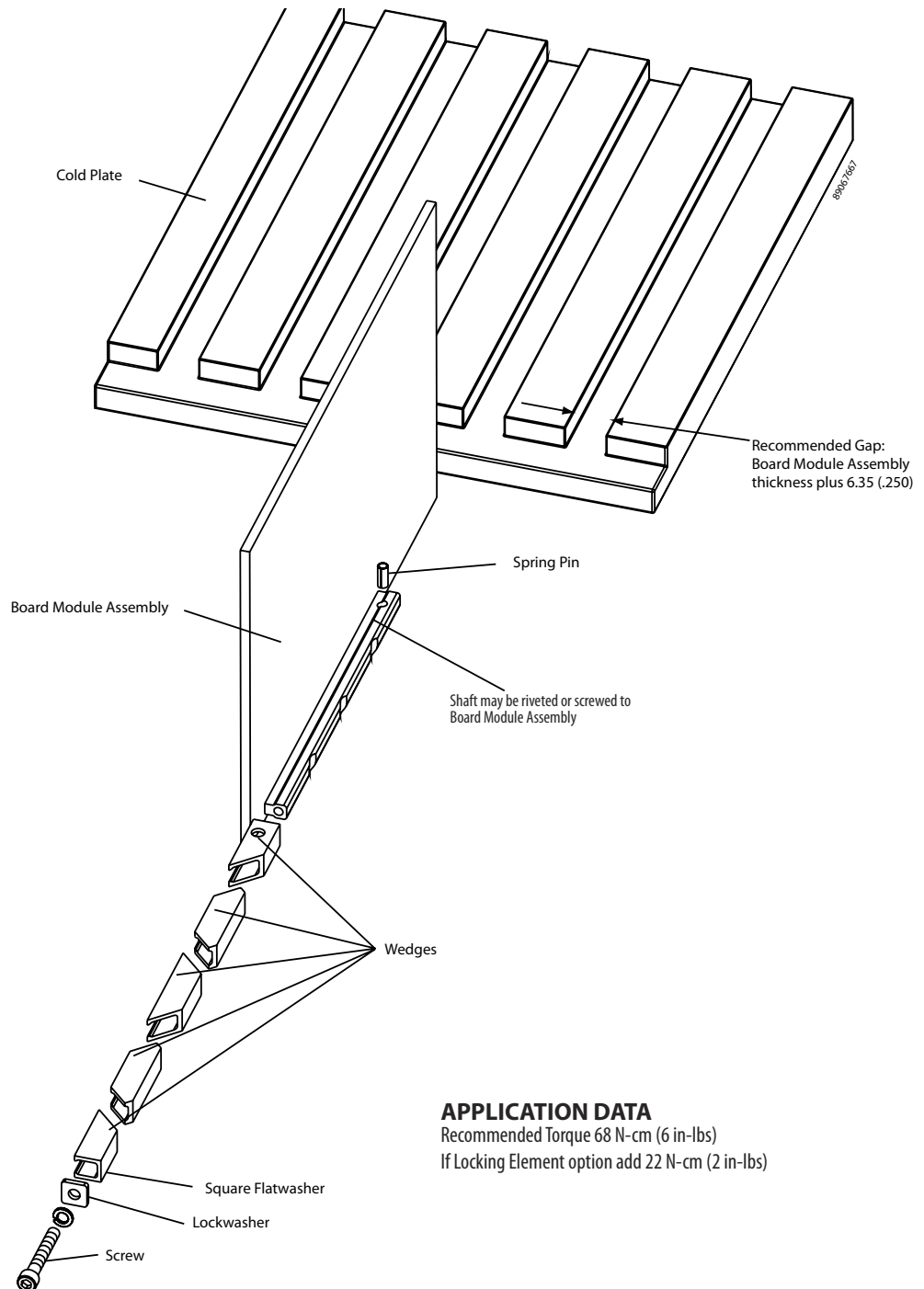
Series 265 "Card-Lok" Retainer (cold plate)
