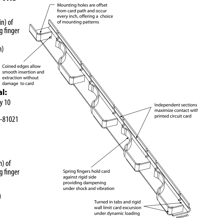
Series 125/126/165/166 retainers
