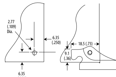
Detail of Actuating Surfaces Required on Top and Bottom Guide Plates
