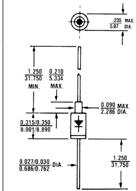
All dimensions in \frac{\text{INCH}}{\text{m.m.}} DO-13 (DO-202AA)
