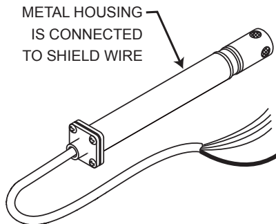
Figure 2.8 Industrial Probe Wiring Hookup
