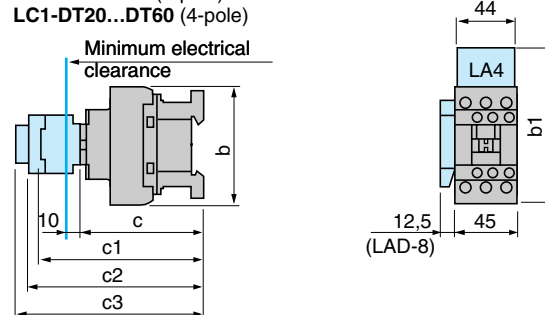
LC1-D25...D38 (3-pole) LC1-DT20...DT60 (4-pole)
