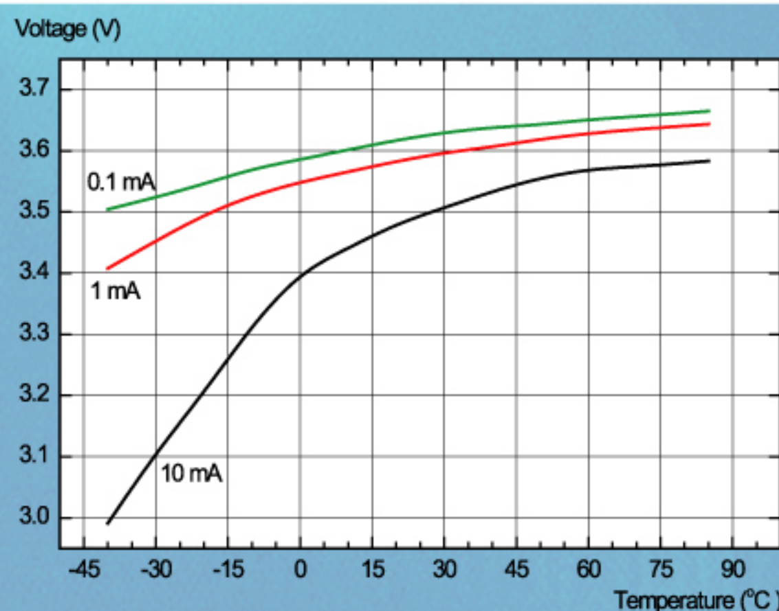
OPERATING VOLTAGE
