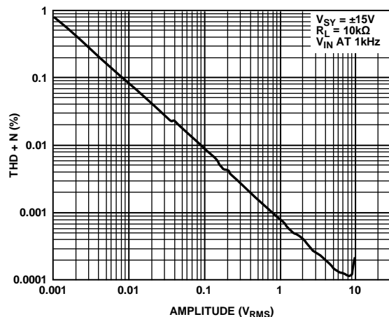
Figure 84. THD + N vs. Amplitude
