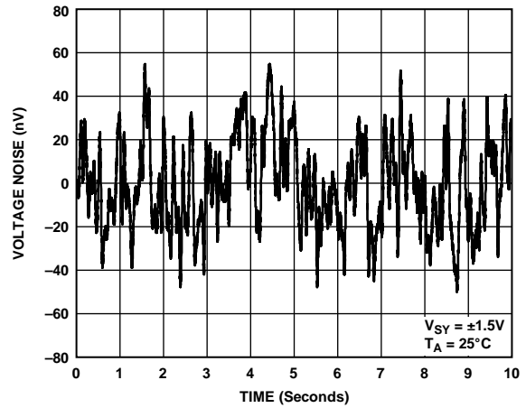
Figure 26. Voltage Noise, 0.1 Hz to 10 Hz
