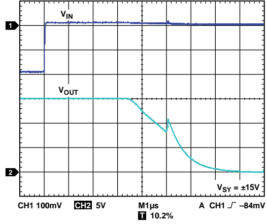
Figure 87. Positive Overload Recovery
