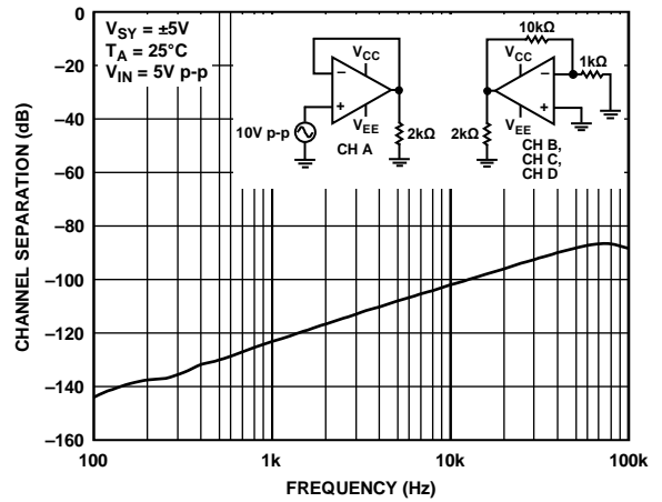
Figure 55. Channel Separation
