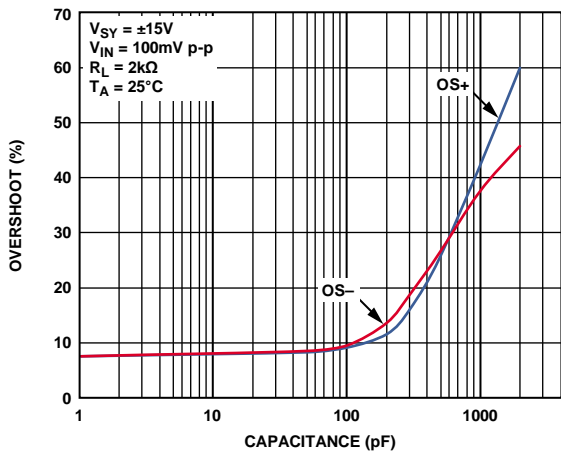
Figure 81. Overshoot vs. Load Capacitance
