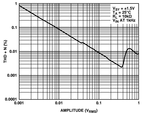
Figure 28. THD + N vs. Amplitude
