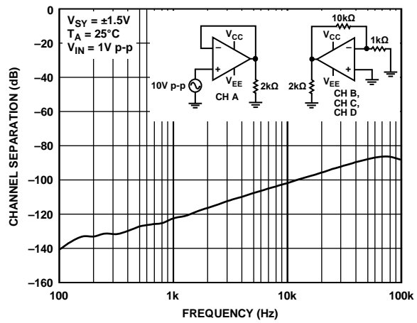
Figure 27. Channel Separation
