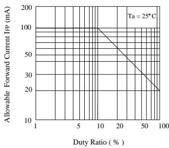
Duty Ratio vs. Allowable Forward Current
