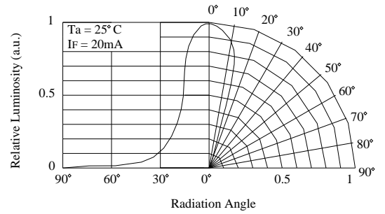
Directivity (Angle : 30^\circ )
