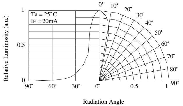
Directivity (Angle : 25^{\circ} )
