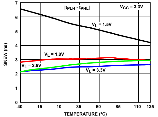
FIGURE 29. ISL3227XE RECEIVER SKEW vs TEMPERATURE
