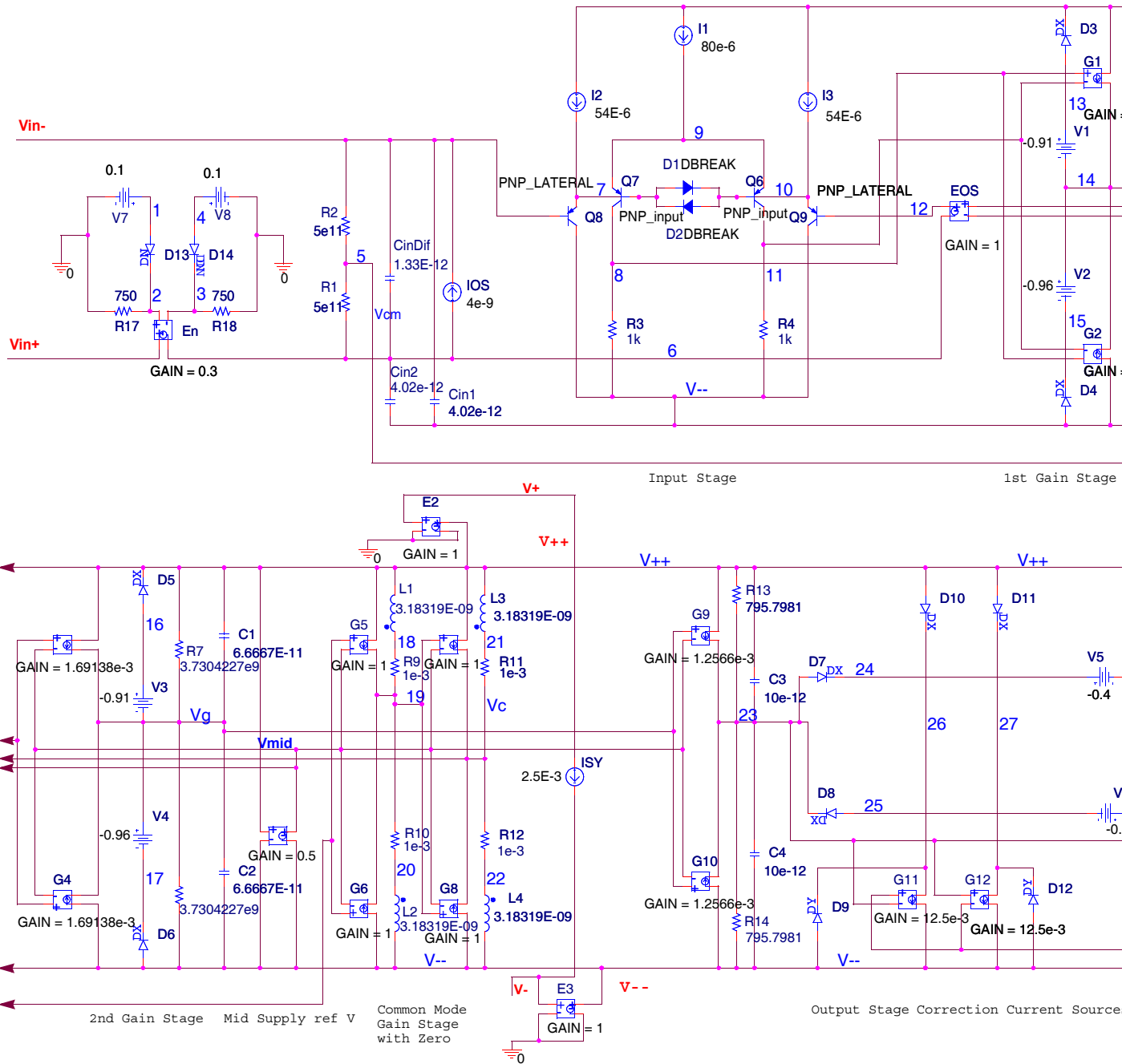
FIGURE 64. SPICE SCHEMATIC
