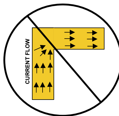
FIGURE 43. AVOID ROUTING ORTHOGONAL CONNECTIONS FOR TRACES THAT HAVE HIGH CURRENT FLOWS
