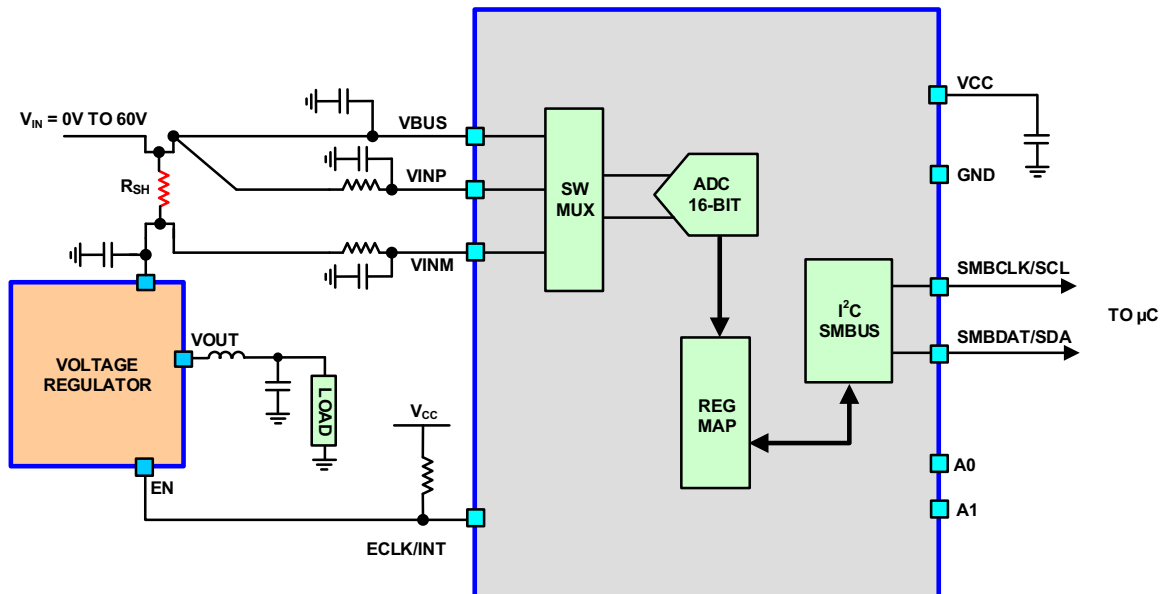
FIGURE 1. TYPICAL APPLICATION
