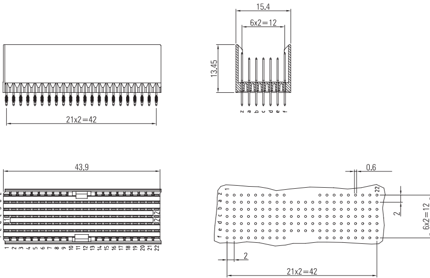
Hole pattern
