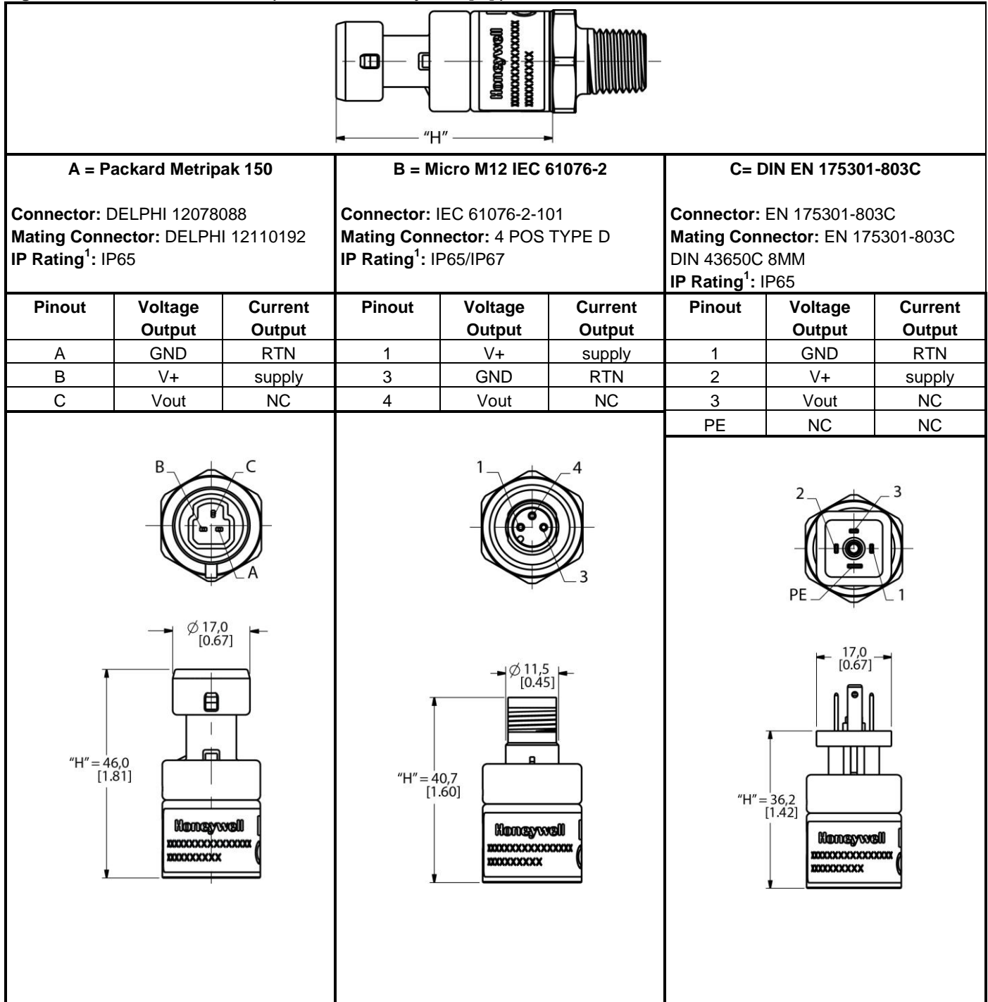
Figure 7. Connector Dimensions (For reference only: mm/[in.] )
