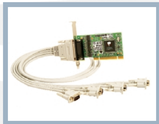
■ INTASHIELD IS-400 4 PORT RS232 PRODUCT CODE: IS-400 Version 2
