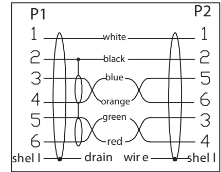
Wire Assignments
