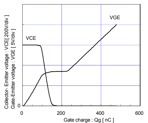
Dynamic Gate charge (typ.) Vcc=600V, Ic=100A, Tj=25°C
