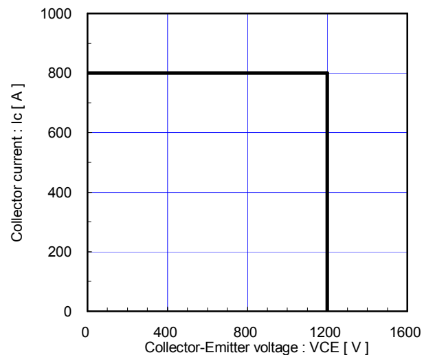
Reverse bias safe operating area (max.) +V_{GE}=15V, -V_{GE} \leq 15V, R_G \geq 1.5\Omega, T_j \leq 125^\circ C
