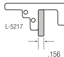
Gripper pads are available in your choice of either parallel, file or grit-type. File-type pads may be used on hard-to-grip insulations.
