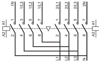
Electrical interlocking of reversers with: mechanical interlock LA9F••• without integrated electrical contacts
