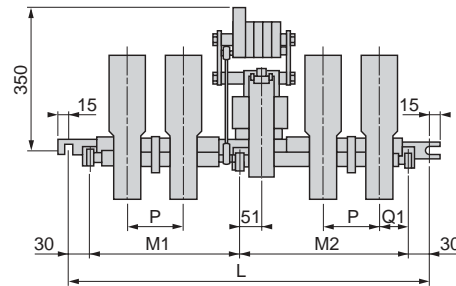
4-pole contactors
