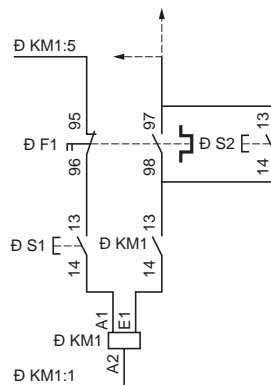
Contactors CR1F
