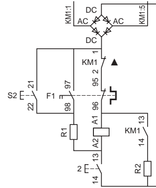
Contactors CR1B
