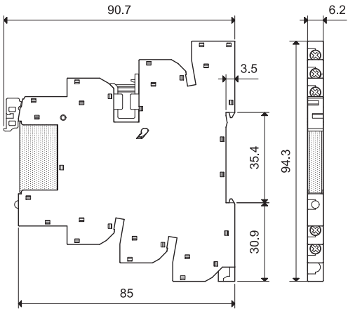
39.80 39.81 Screw terminal
