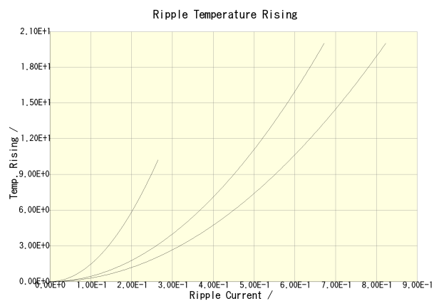
CKCA43X7R1E473M100AA(100kHz) CKCA43X7R1E473M100AA(500kHz) CKCA43X7R1E473M100AA(1MHz)
