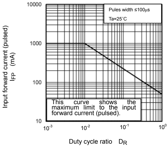
I_{FP} - D_R
