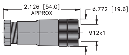
Female Connector
