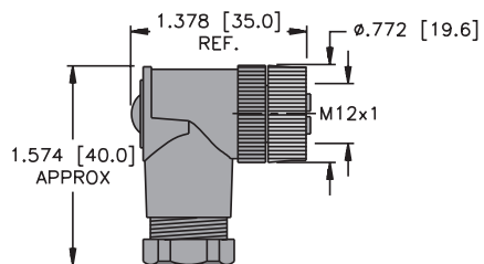
Female Connector
