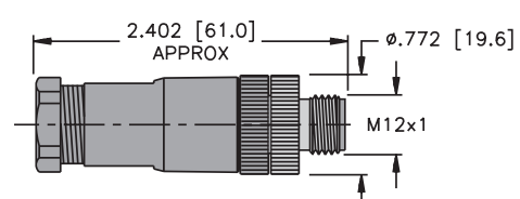
Male Connector
