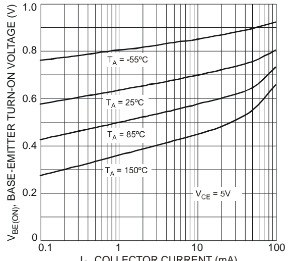
Fig. 5 Typical Base-Emitter Turn-On Voltage vs. Collector Current
