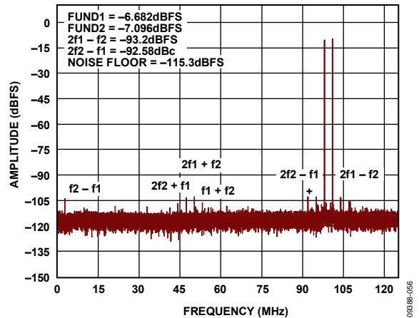
Figure 57. Measured Two-Tone Performance of the Circuit Shown in Figure 54 for a 100 MHz Input Signal
