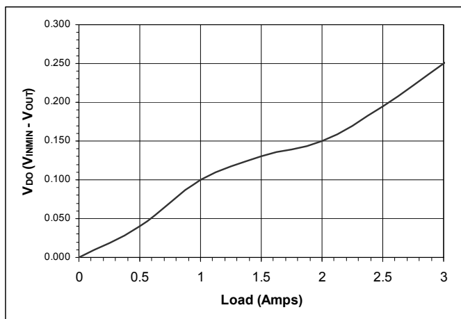
Drop-Out Voltage
