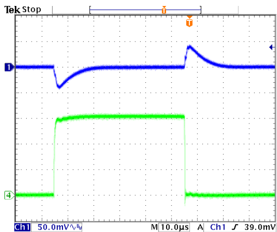
Load Transient: V_{IN} = 5.0V , V_{OUT} = 1.2V Ch.1: V_{OUT} , Ch.4: I_{LOAD} (slew rate \geq 10A/\mu S ) C_{IN} = 22\mu F , C_{OUT} \approx 50\mu F
