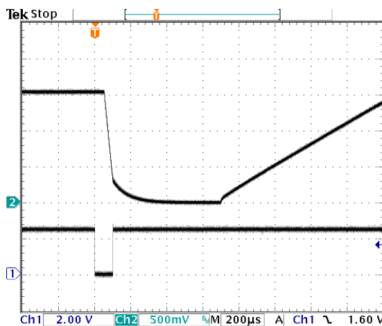
Enable Lock-out Time, Ch.1: ENABLE, Ch. 2: V_{OUT}
