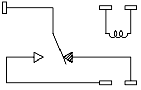
WIRING DIAGRAM
