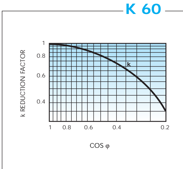
Load reduction factor vs cos φ.
