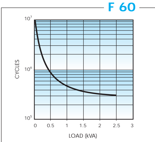
Contact life vs AC1 load at 1800 cycles/h.
