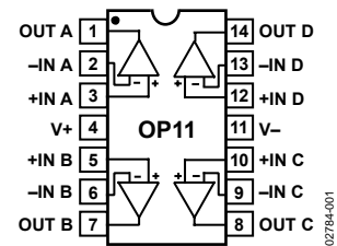
Figure 1. 14-Lead PDIP (N-14) (P Suffix)
