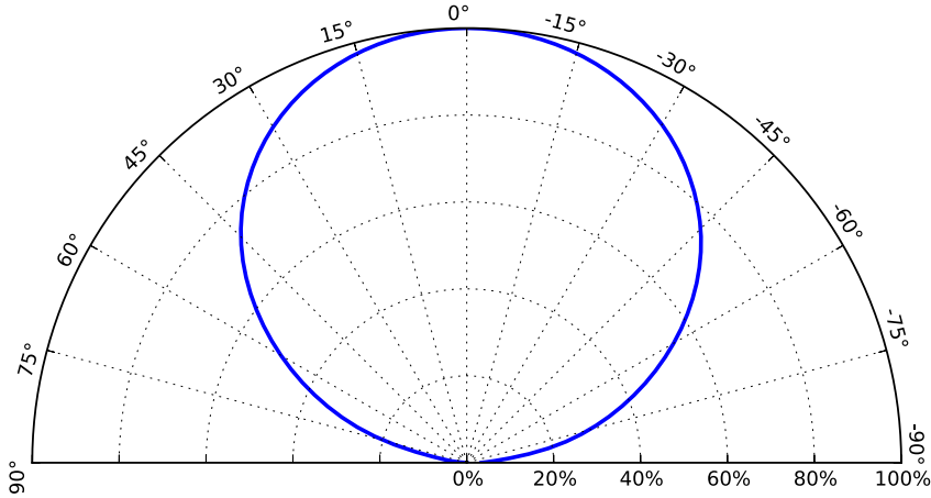
Figure 4b: Typical polar radiation pattern for LXHx-FWxx at 700mA, T_j=85^\circ\text{C} .
